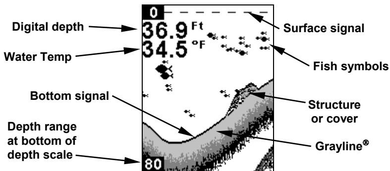
Full Chart page.
