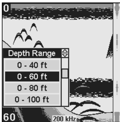
Depth Range menu with Manual setting selected (left). Range menu with 0-60 ft highlighted (right).
