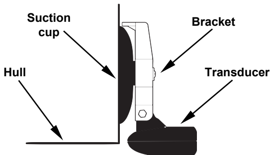
Portable transducer installed on boat transom.
