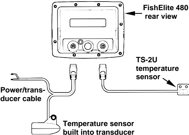
FishElite 480 with secondary external temperature sensor. Primary temp sensor is built into the transducer.
