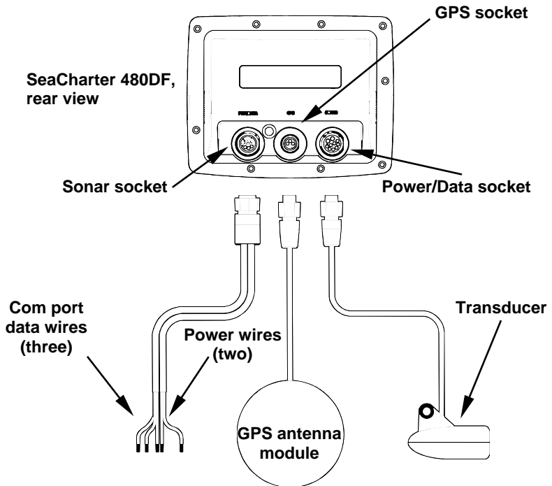
SeaCharter 480DF cable connections.
