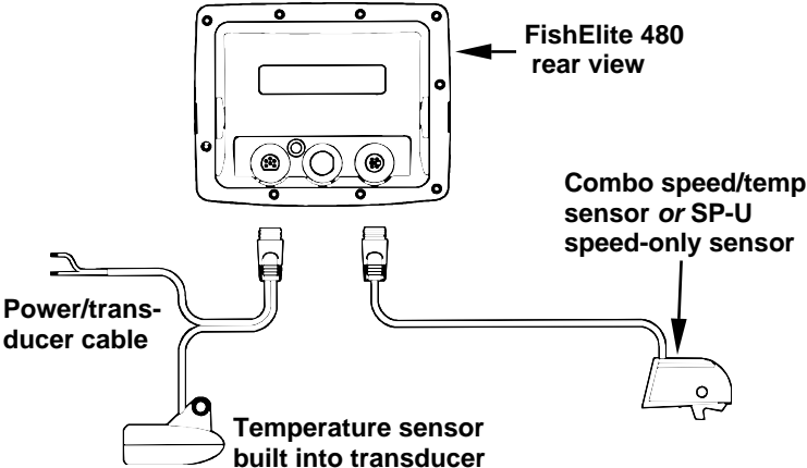
FishElite 480 with external speed sensor or combo speed/temp sensor. The primary temperature sensor is built into the transducer.
