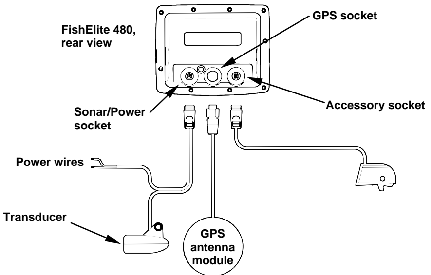
FishElite 480 cable connections.
