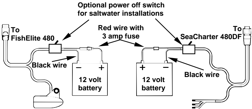
Power connections for the FishElite 480 (shown left) and SeaCharter 480DF (shown right) sonar/GPS units.
