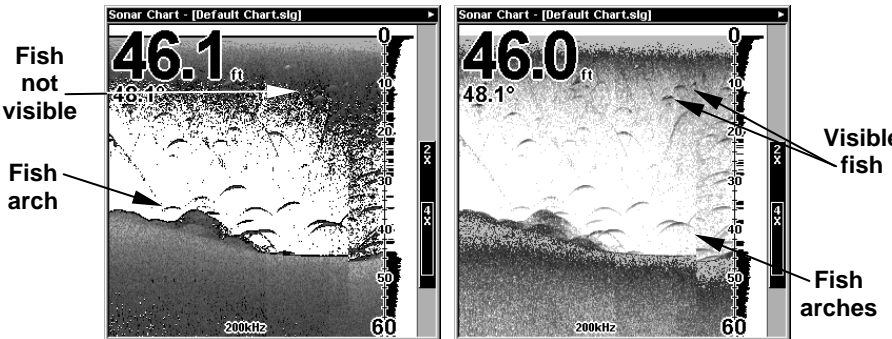
Sonar chart in regular grayscale mode, left, and in FishReveal mode, right. Notice how shallow fish formerly hidden in the surface clutter become visible in FishReveal mode.
