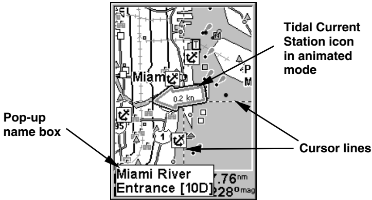
Navionics chart showing Tidal Current Station icon selected by cursor. In this example, the current is flowing to the west at 0.2 kn.
