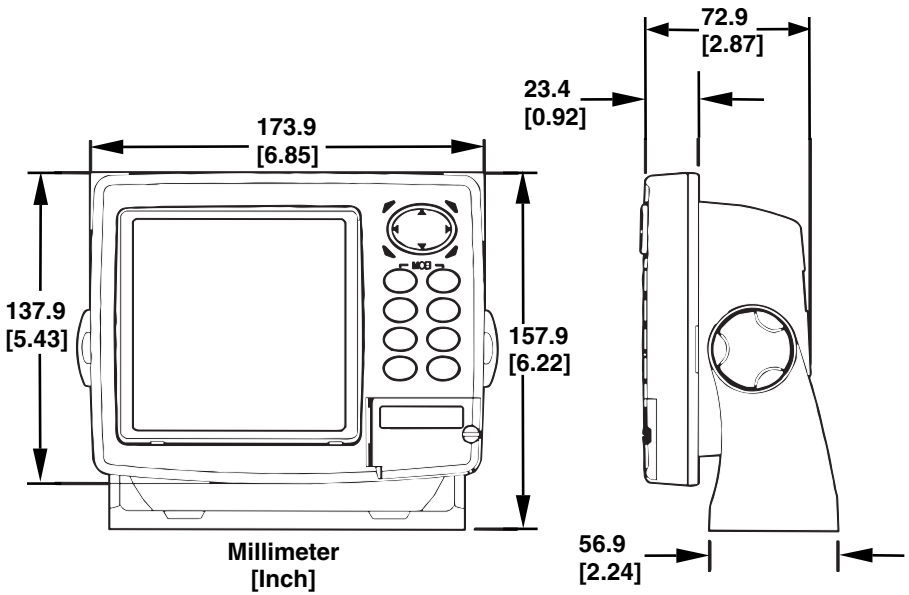
Front view (left) and side view (right) showing dimensions of the sonar unit when mounted on gimbal bracket.
