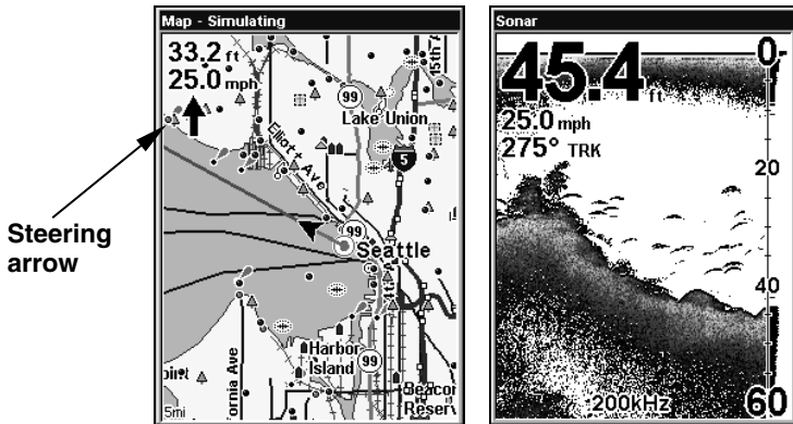
At left, Map Page showing boat cruising Puget Sound, Washington, with Overlay Data turned on. This example shows Depth, Ground Speed and the Steering Arrow. Note the Steering Arrow always points directly to the destination you are navigating toward. Right, the example shows Depth, Ground Speed and the Track the boat is following.
