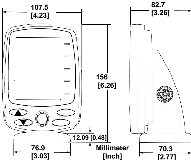
Front view (left) and side view (right) showing dimensions of the FishEasy 320C when mounted on quick release bracket.
