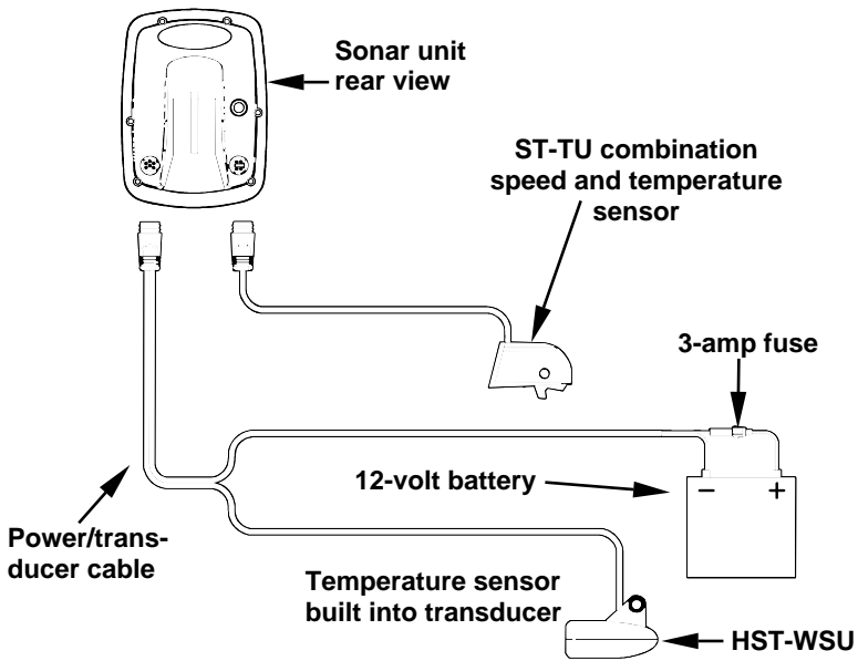
Sonar unit with external combination speed and temperature sensor. Primary temp sensor is built into the transducer.
