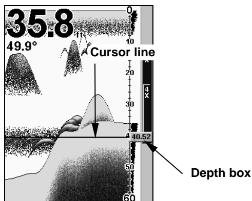
Sonar chart with the depth cursor active. The line indicates the large fish is 40.52 feet deep.
