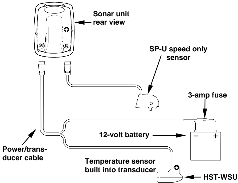
Sonar unit with external speed sensor. The temperature sensor is built into the transducer.
