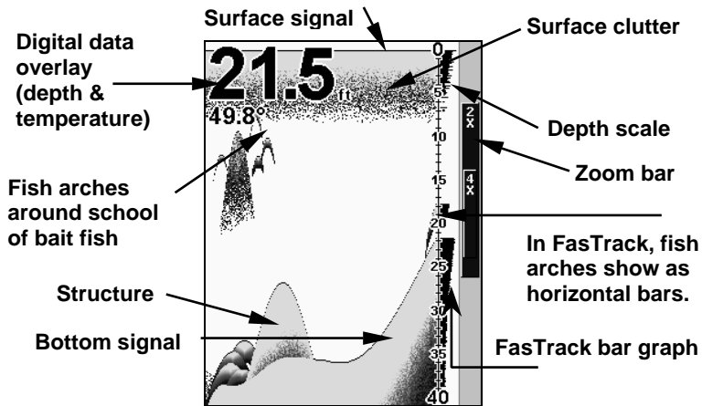
Sonar Page, showing full sonar chart mode.
