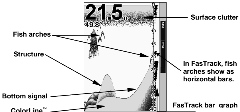
Sonar Page showing FasTrack.
