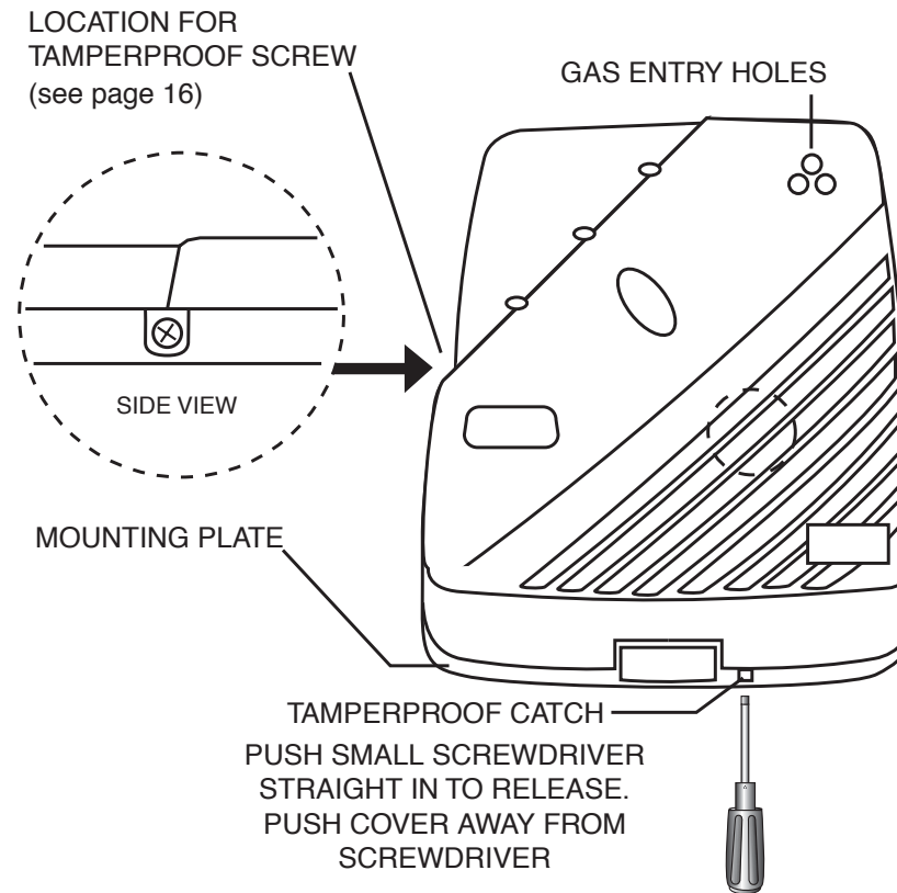
Figure 4 - Alarm Installation
