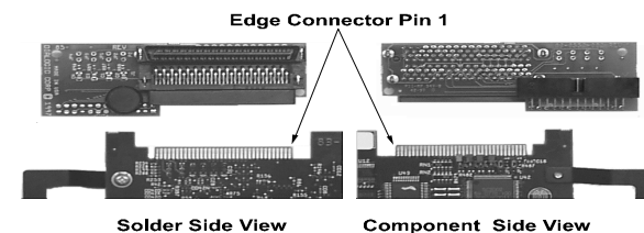
Figure 2. Adapter Alignment (D/41ESC-PCI shown)
