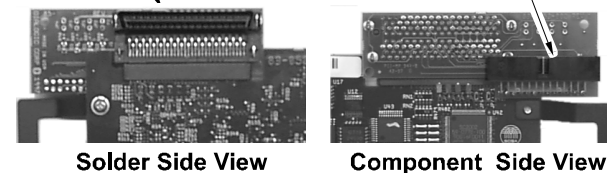
Figure 3. Connect the Adapter (D/41ESC-PCI shown)
