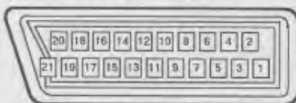
21-PIN TERMINAL
