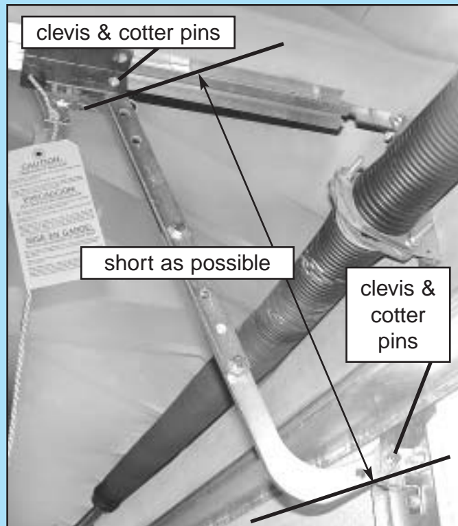
FIG. 2-10 Attaching door arms (sectional doors).
