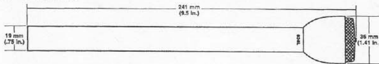
FIGURE 2 — Dimensions
