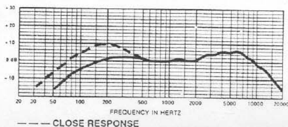
FIGURE 1 — Frequency Response
