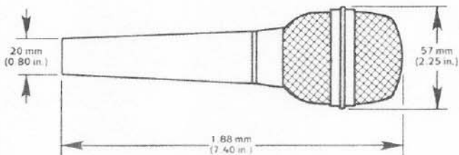
FIGURE 3 Dimensions
