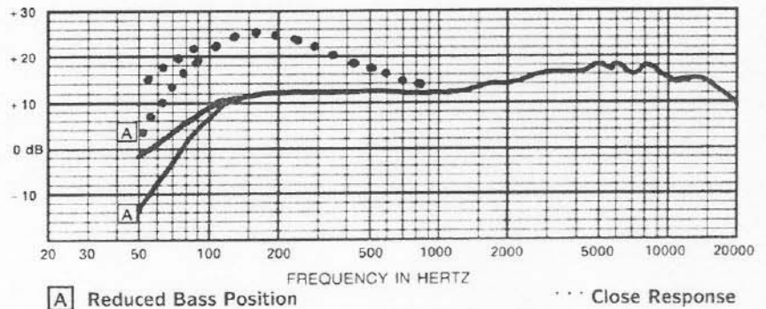
FIGURE 1 Frequency Response
