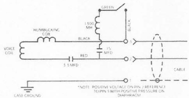
FIGURE 4 Wiring Diagram
