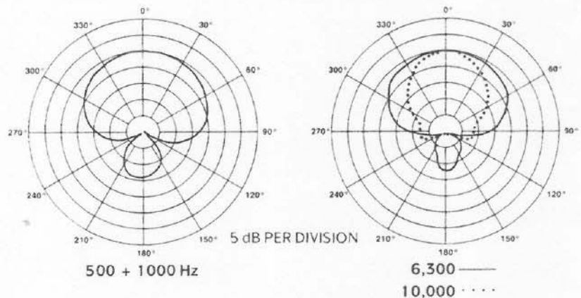
FIGURE 2 Polar Response
