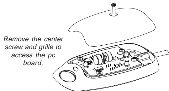
Figure 2: PCB Access
