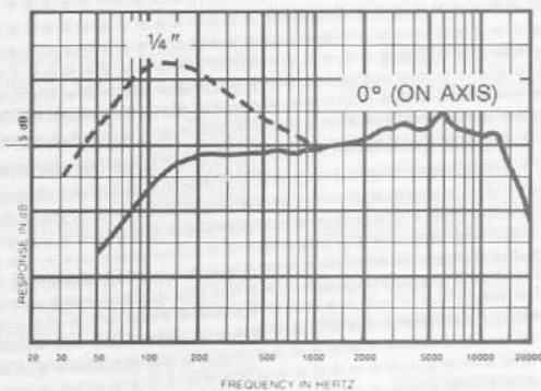
FIGURE 3 — Frequency Response
