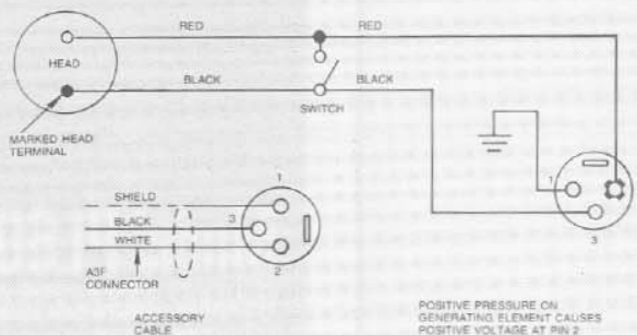
FIGURE 2 — Wiring Diagram
