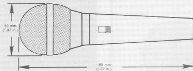
FIGURE 1 — Dimensions
