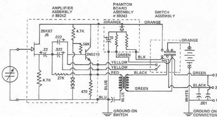
FIGURE 2 - Wiring Diagram
