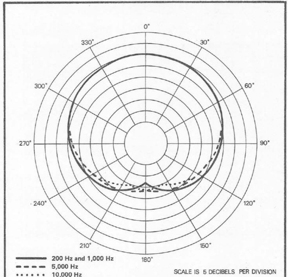
FIGURE 4 – Polar Response
