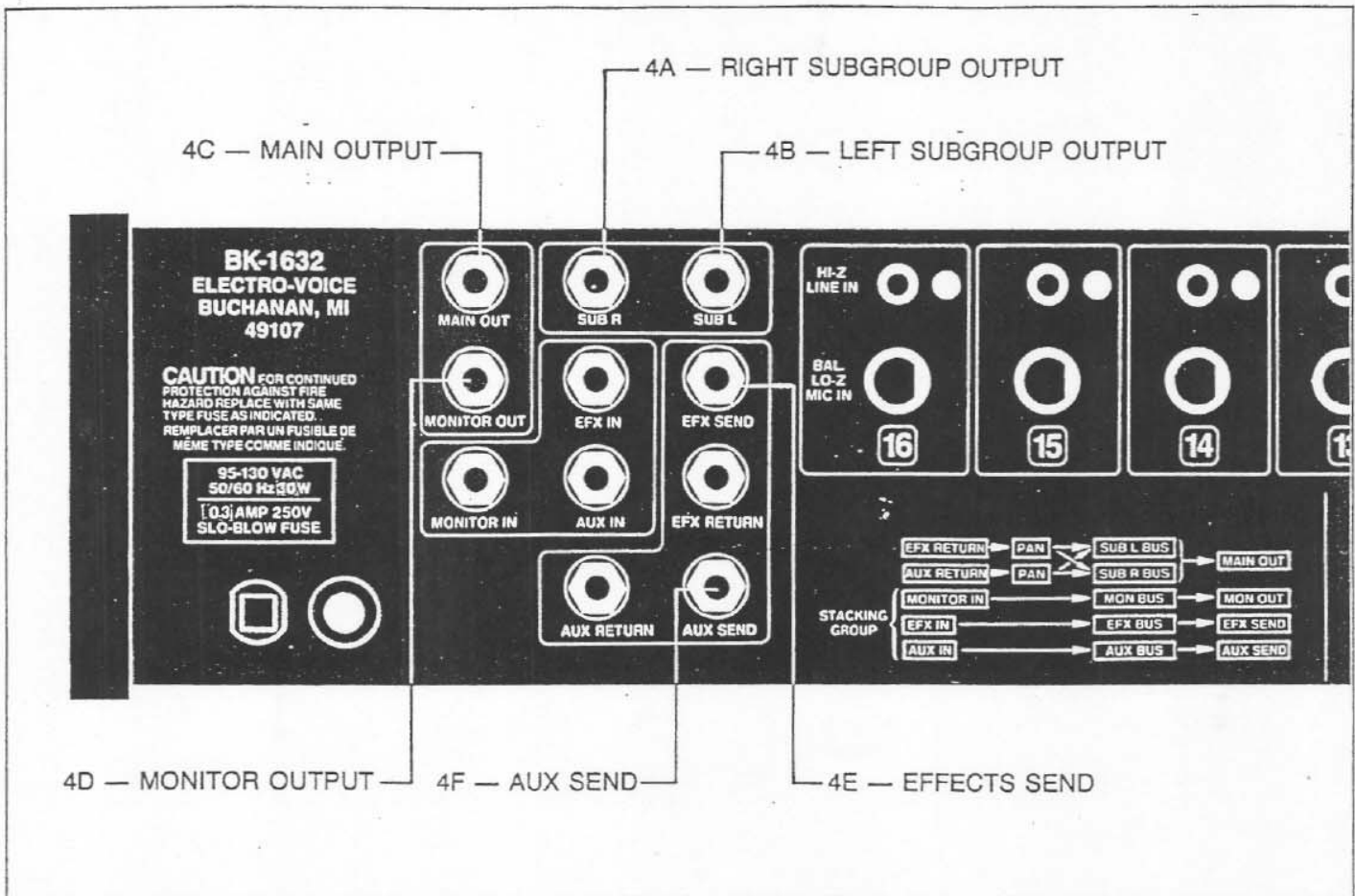
FIGURE 4 — Output Jacks
