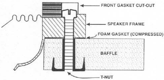
FIGURE 4 — Rear-Mounting Detail (not to scale)
