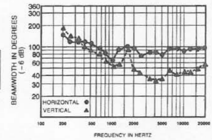
FIGURE 3 MTH-2/94A Beamwidth vs. Frequency
