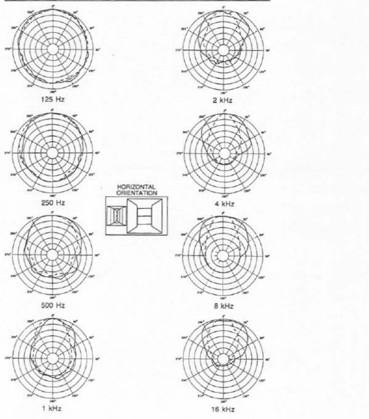
FIGURE 2 - MTH-2/94A Polar Response (1/2-octave 4 volts at 20 feet nominal)
