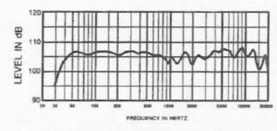
FIGURE 5 - MTH-2/94A Axial Frequency Response using Recommended Crossover, Equalization, Time Delay and MTL-2 Low-Frequency System
