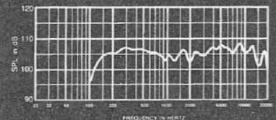
FIGURE 1 Axial Frequency Response using Recommended Crossover, Equalization 1 Watt/1 Meter into MB Section
