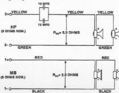
FIGURE 7 — Wiring Diagram
