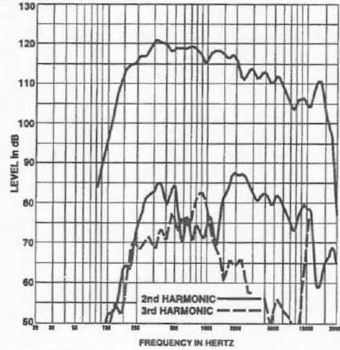
FIGURE 6 — Harmonic Distortion
