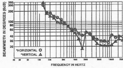
FIGURE 4 — MTH-2.5/22B Beamwidth vs. Frequency
