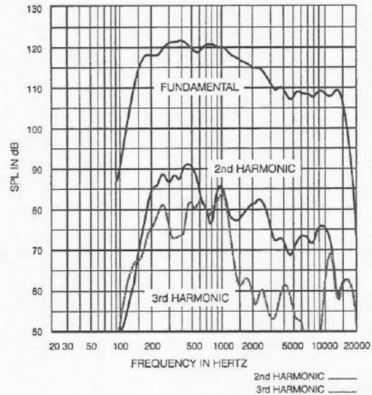
FIGURE 6 — MTH-2.5/22B Harmonic Distortion
