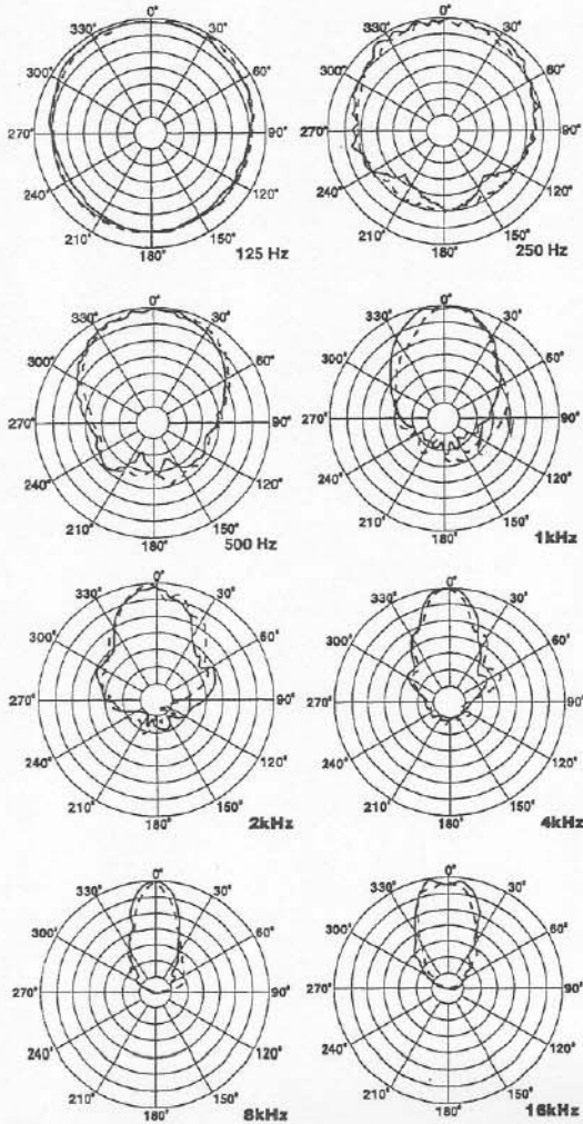
FIGURE 3 — MTH-2.5/22B Polar Response
