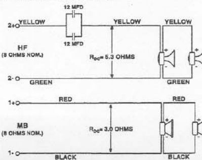
FIGURE 7 — MTH-2.5/22B Wiring Diagram
