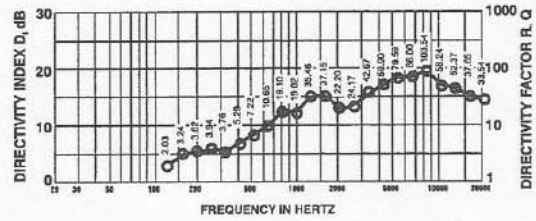
FIGURE 5 — MTH-2.5/22B Directivity vs. Frequency
