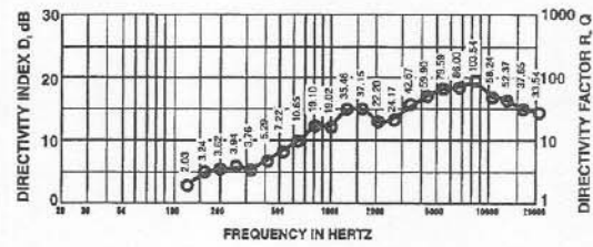
FIGURE 5 — MTH-2.5/22BT Directivity vs. Frequency
