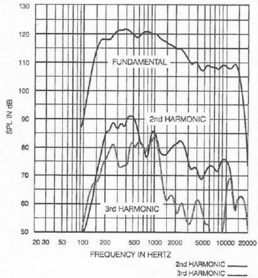
FIGURE 6 — MTH-2.5/22BT Harmonic Distortion
