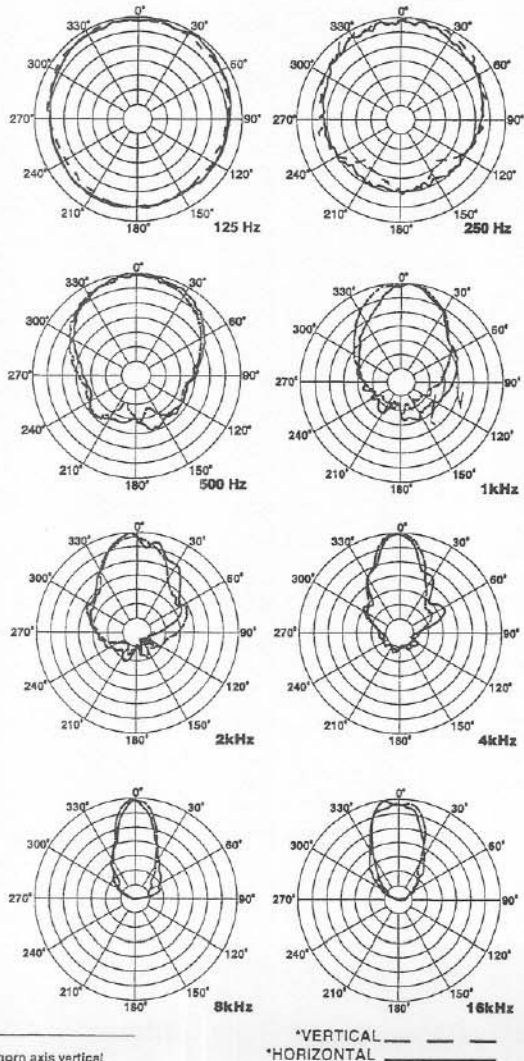
FIGURE 3 — MTH-2.5/22BT Polar Response
