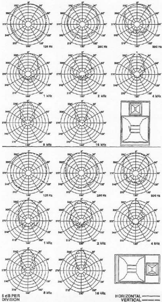
FIGURE 3 — Polar Response
