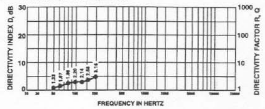
FIGURE 5 — Directivity vs. Frequency
