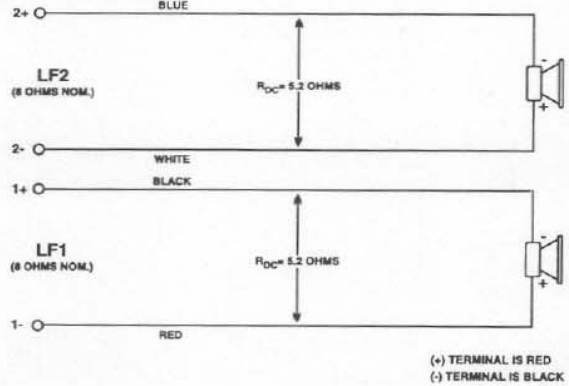
FIGURE 7 — Wiring Diagram
