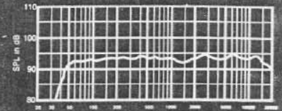
FIGURE 1 Axial Frequency Response 4 Volts/10 Feet
