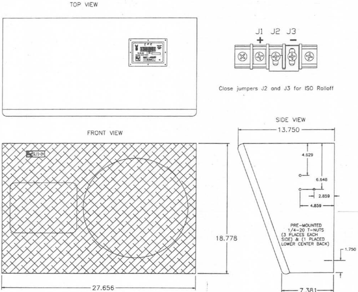
Figure 6—SL15-2H Dimensions and ISO Selection
