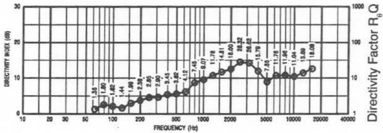
Figure 4—Directivity vs. Frequency (anechoic environment)
