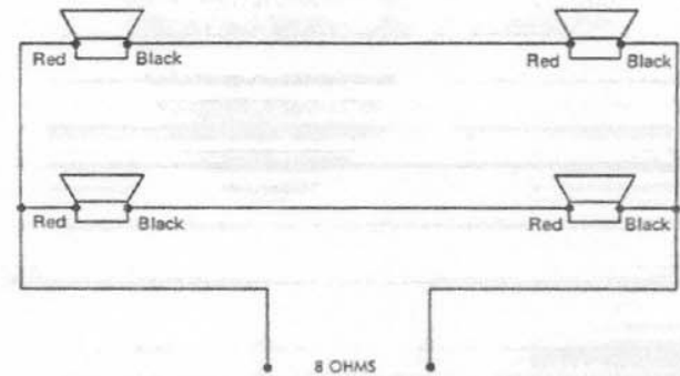
Figure 3 - Connection of four SRO/12 speakers in series-parallel
