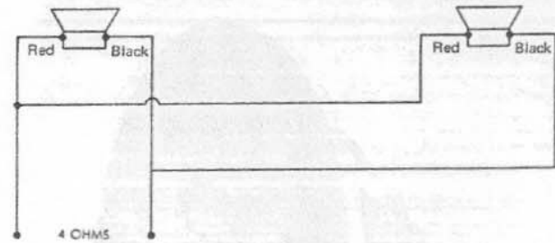
Figure 2 - Connection of two SRO/12 speakers in parallel
