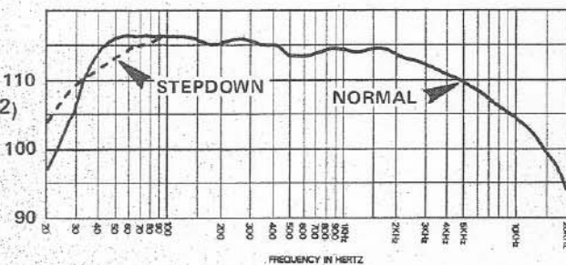
FIGURE 5 — Maximum Acoustic Output
