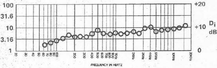
FIGURE 2 — Directivity vs Frequency
