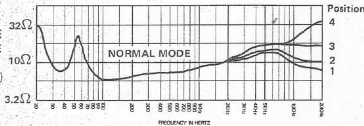
FIGURE 4 — Impedance vs Frequency
