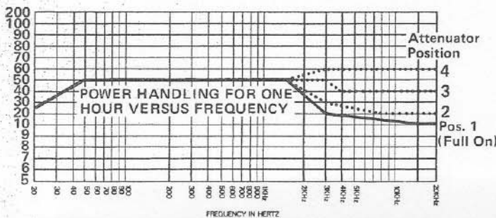
FIGURE 6 — Power Handling Chart (average sine wave power, nominal 8 ohm load)
