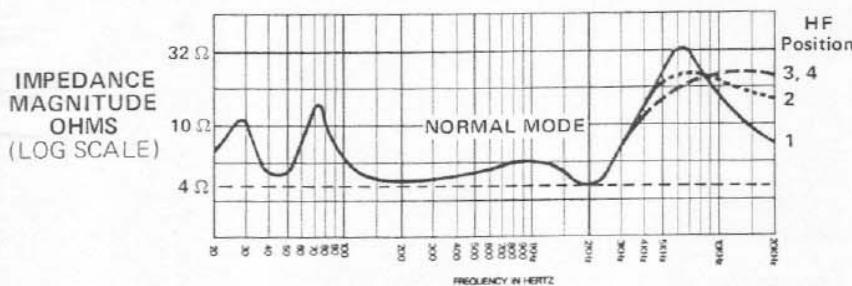
FIGURE 4— Impedance vs Frequency
