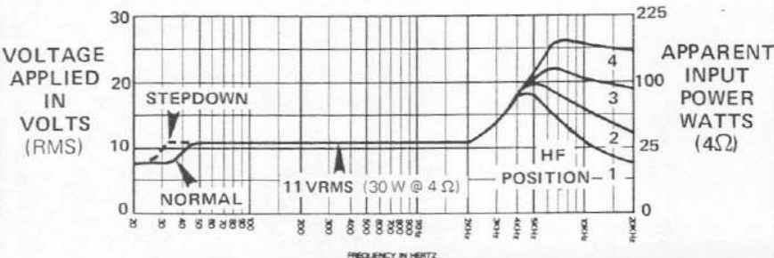
FIGURE 6— Maximum Sinewave Power Input
