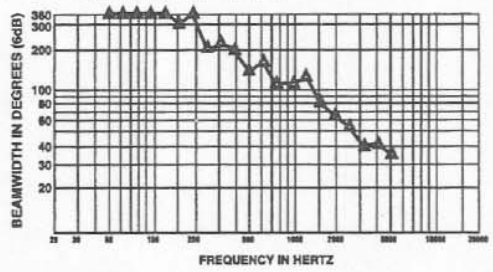
FIGURE 8 — Directivity vs. Frequency
