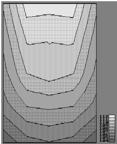
EASE™ Direct Field SPL
