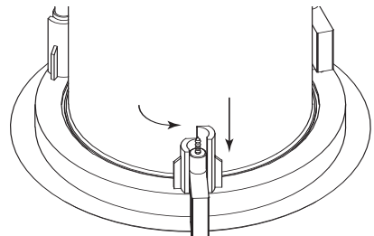
Figure 17: Tighten mounting tabs
