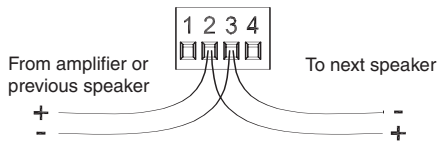
Figure 9: Parallel wiring
