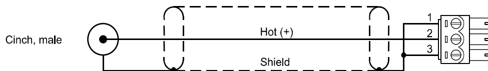
N8000 Digital (unbalanced) audio input cable, Cinch (male) on Phoenix
