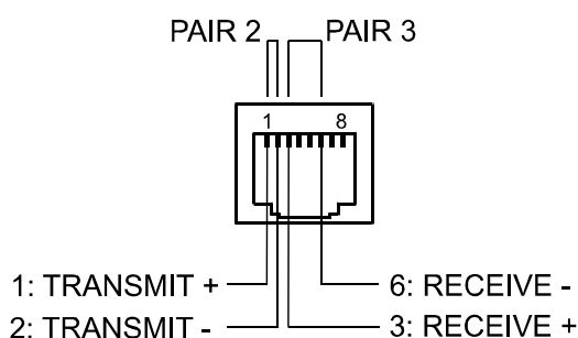
Pin Assignment of Ethernet jack
