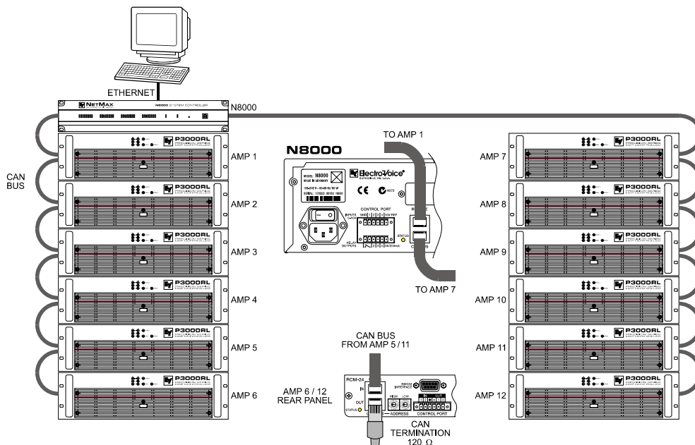
System with 2 amp-racks and 1 N8000/PC in the middle. Termination plugs at power amp 6 (first unit on the bus) and power amp 12 (last unit on the bus).
