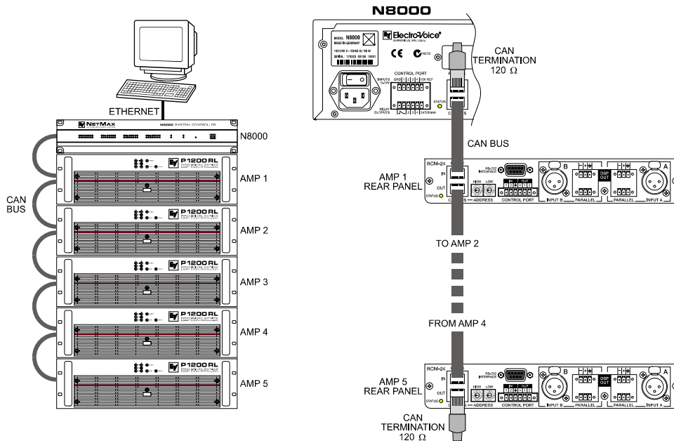
System with 5 power amps and 1 N8000 at the beginning of the bus. Termination plugs at the N8000 (first unit on the bus) and at amp 5 (last unit on the bus).
