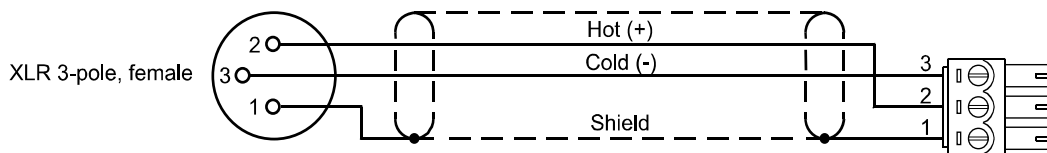
N8000 Digital (balanced) audio input cable, XLR (female) on Phoenix
