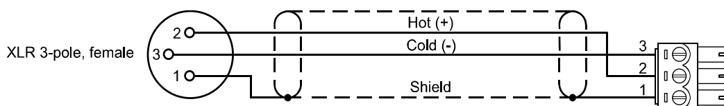
N8000 Analog audio input cable, XLR (female) on Phoenix
