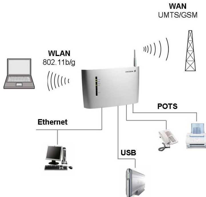
Figure 2 - Overview of Interfaces for the Ericsson W25
