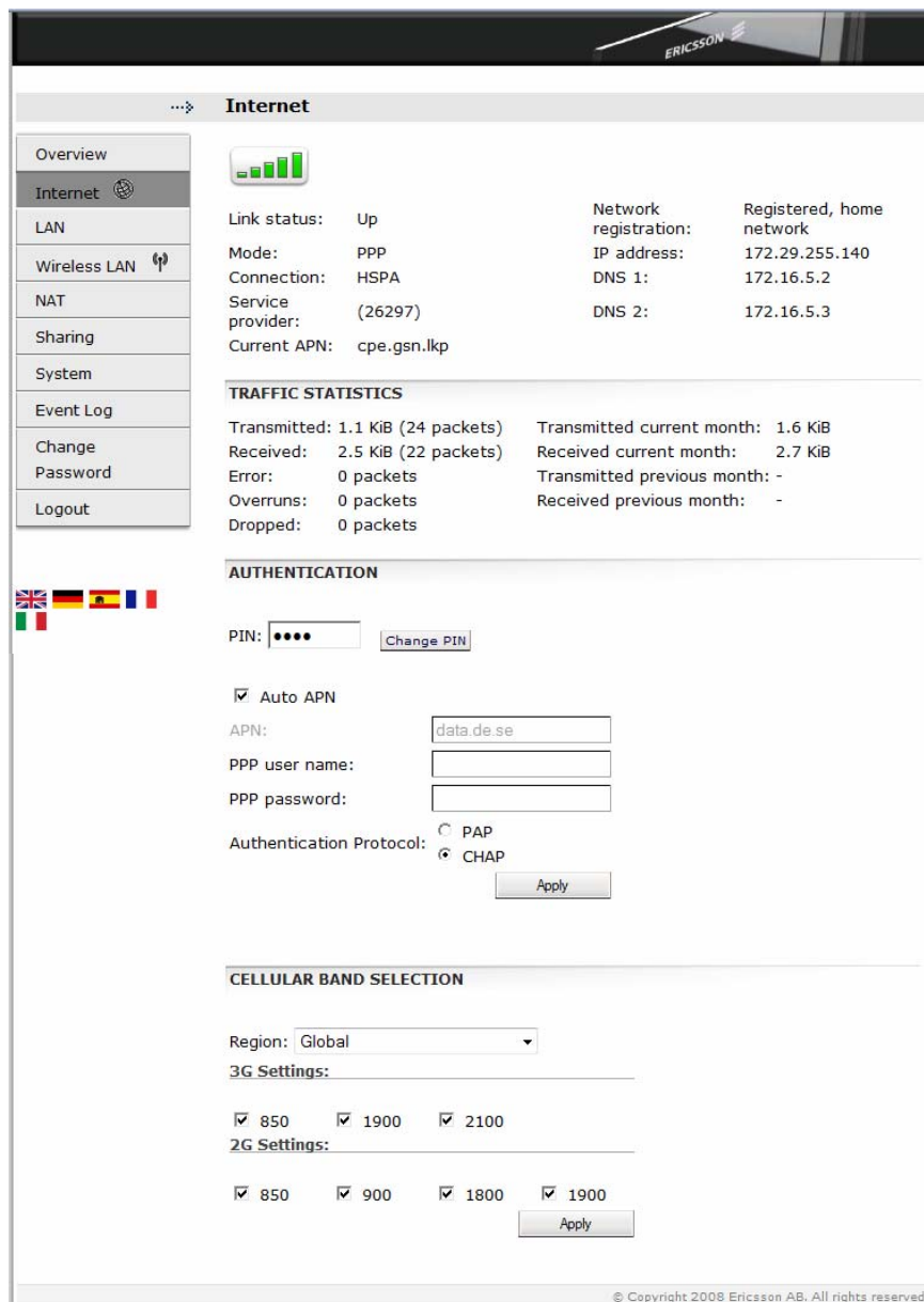
Figure 26 - Internet page
