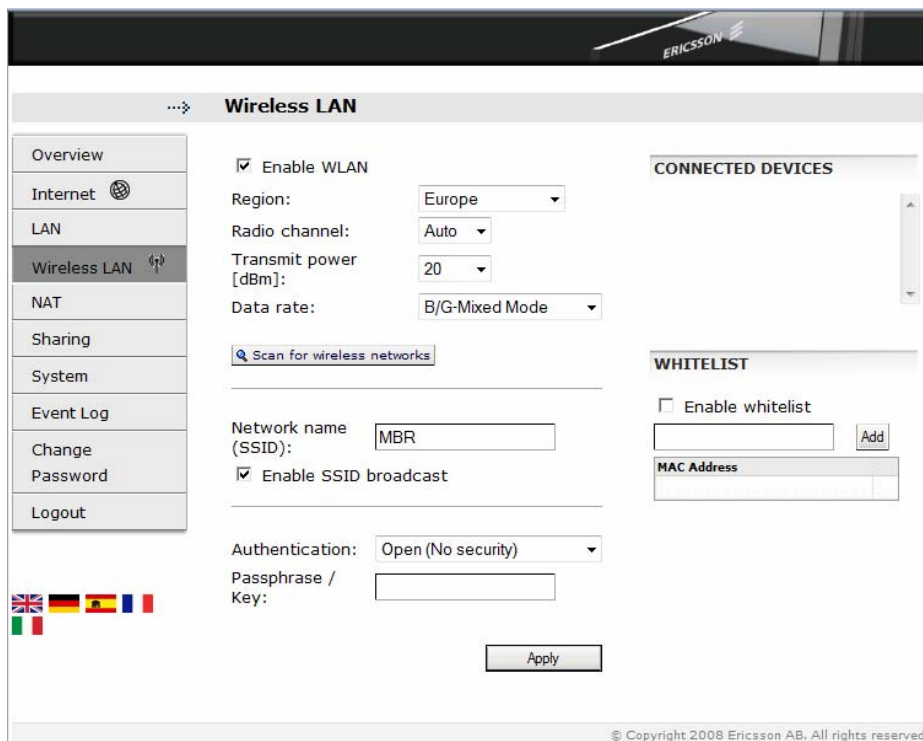
Figure 35 - Wireless LAN page
