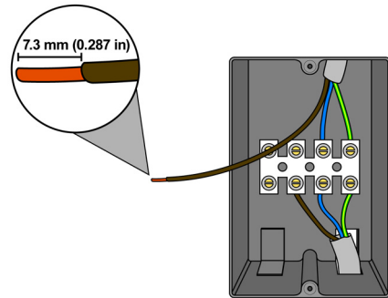
Figure 1. Strip Wire Insulation
