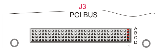
Figure 5. PCI BUS layout
