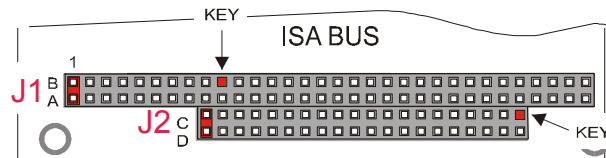
Figure 4. ISA BUS layout
