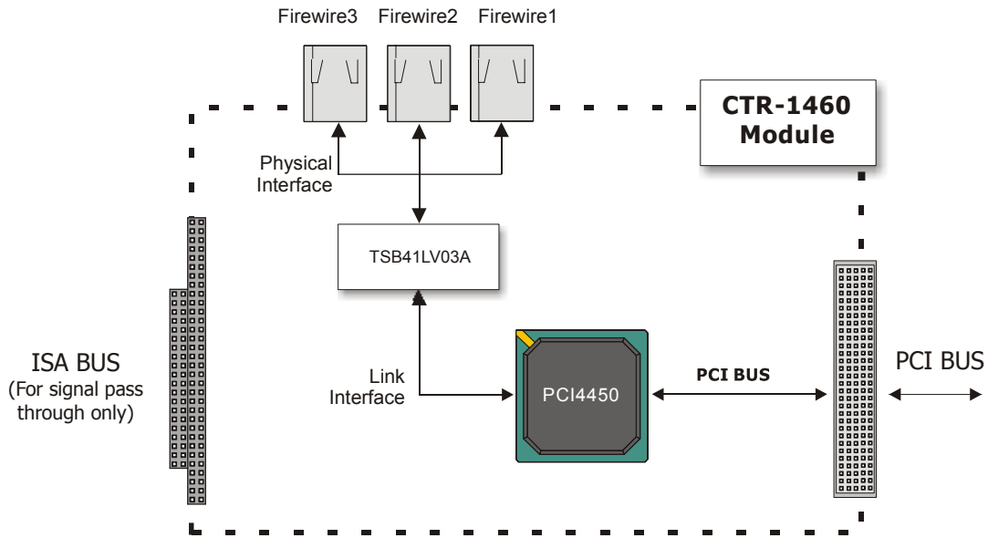
Figure 1. Functional blocks of the COM-1460 module
