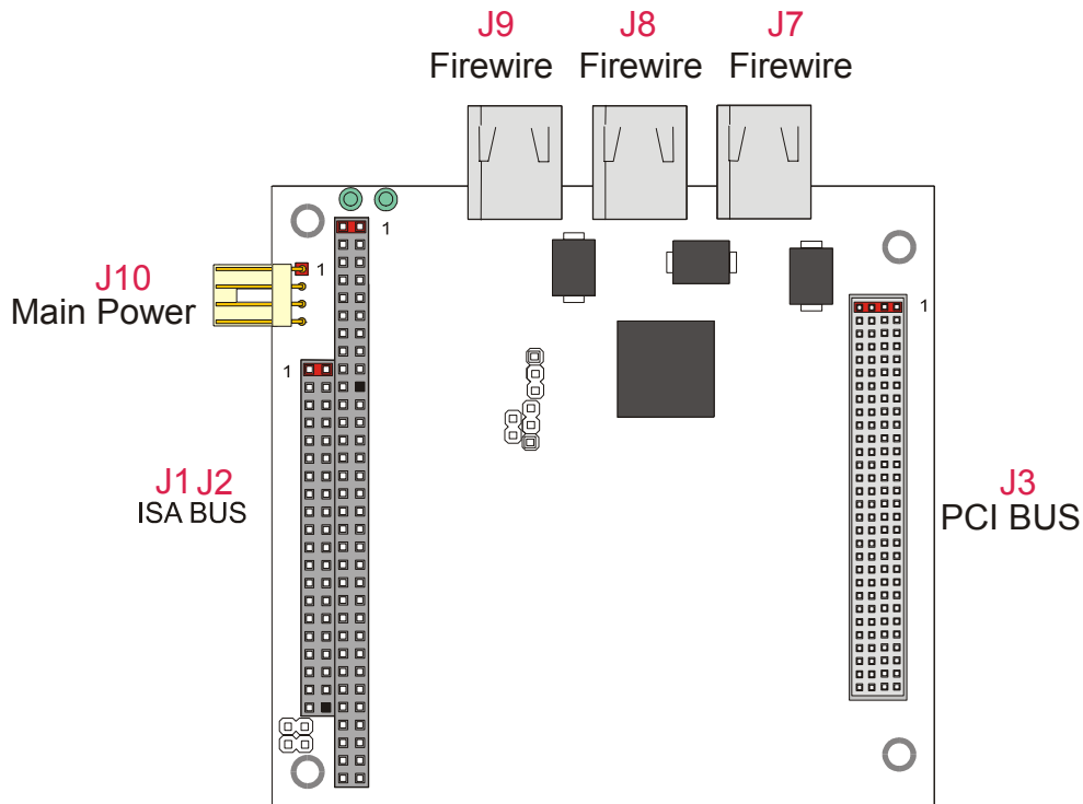
Figure 3. Connectors layout
