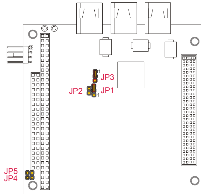
Figure 2. Jumpers on the COM-1460 module
