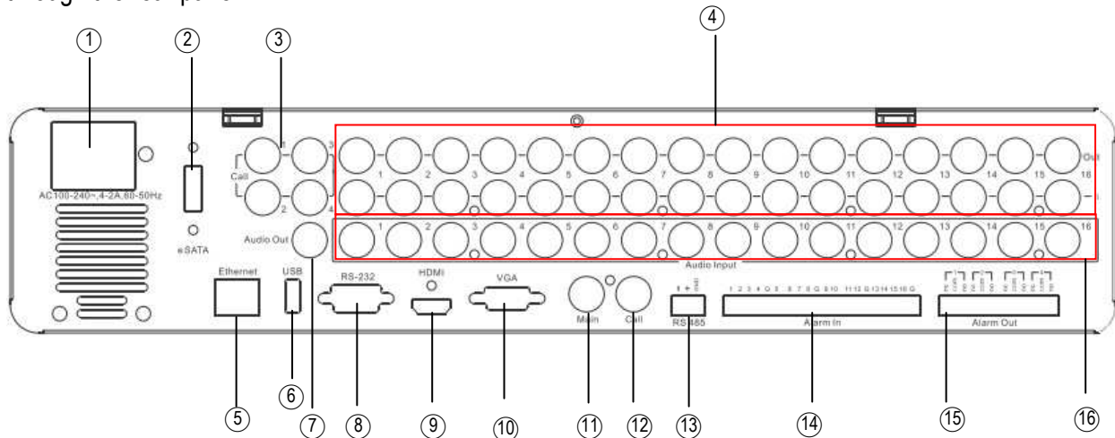
Figure 1-2 Rear Panel
