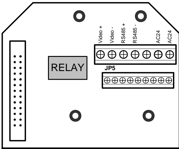
EPTZ500 Baseboard
