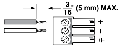
Unbalanced Input
