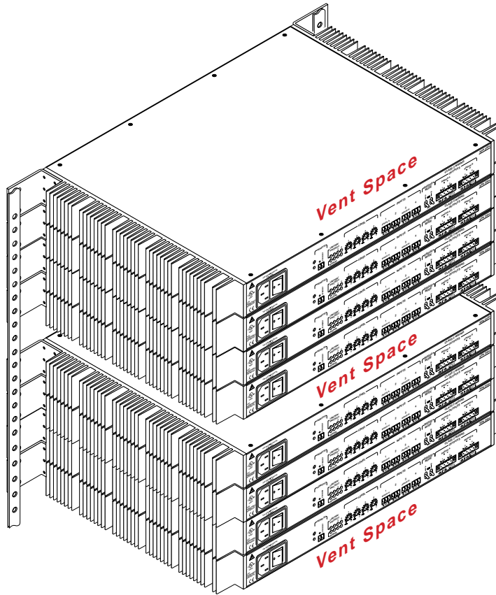
Figure 6. Allow Sufficient Spacing for Adequate Ventilation
