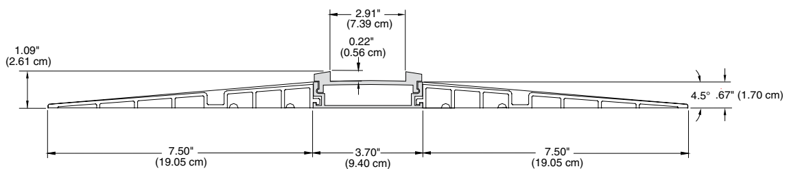
BACK VIEW of AVTrac 4C EXT
