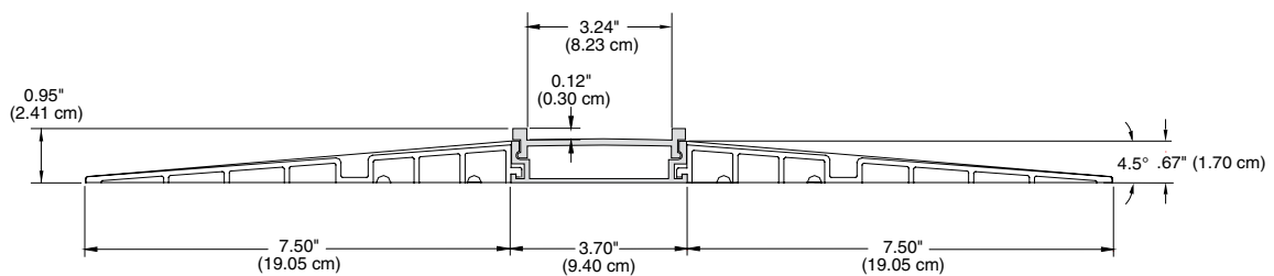
BACK VIEW of AVTrac 4R EXT
