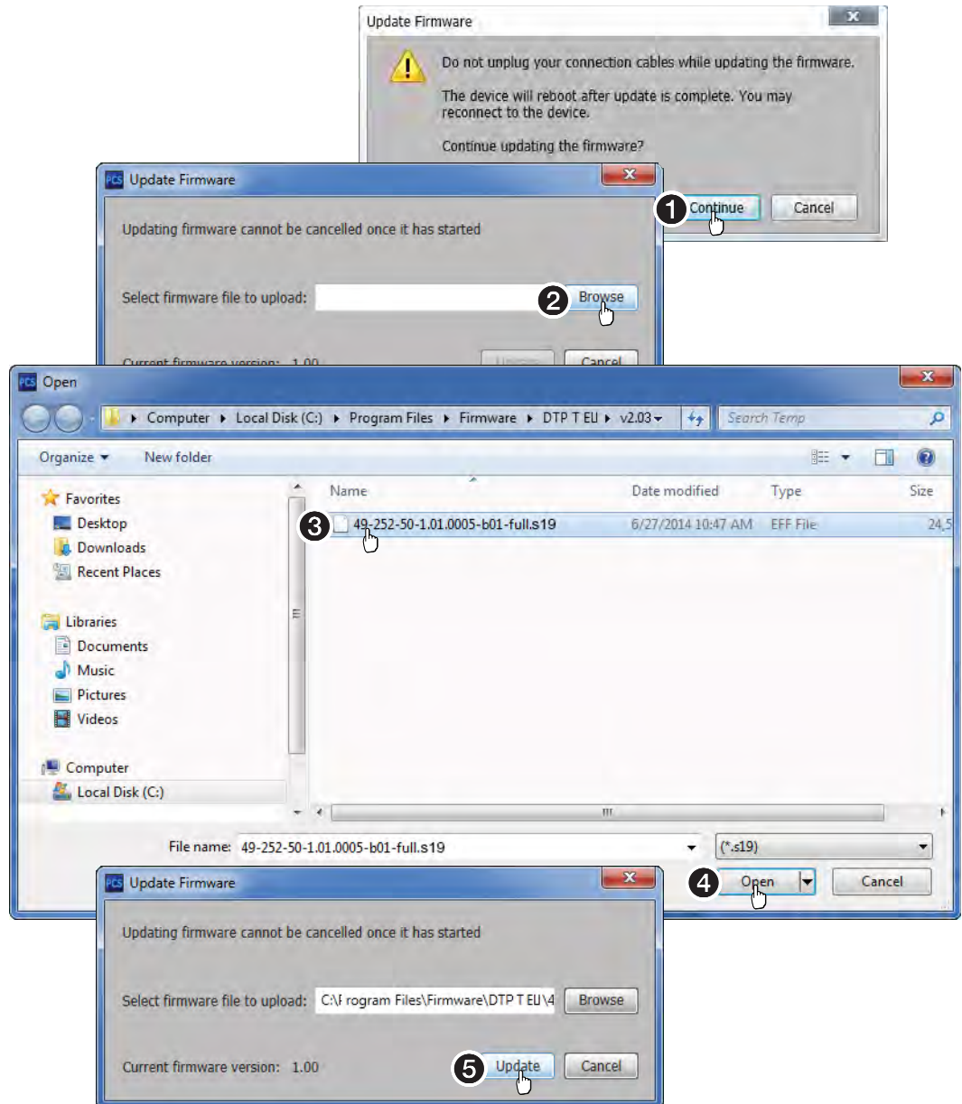
Figure 21. Updating Firmware
