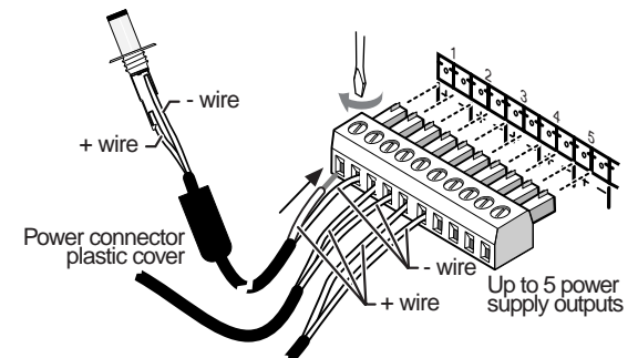
Figure 3 — Connecting power cables to P/S 100
