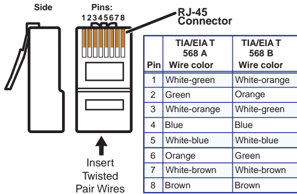
Figure 7. TP Cable Termination
