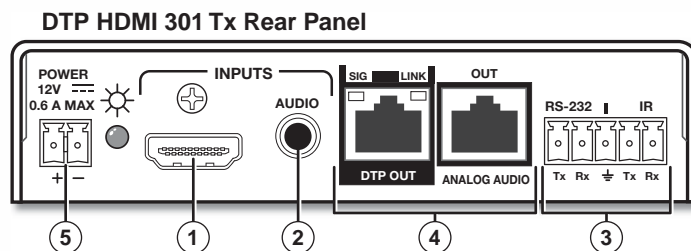
Figure 2. DTP HDMI 301 Tx Rear Panel Connectors
