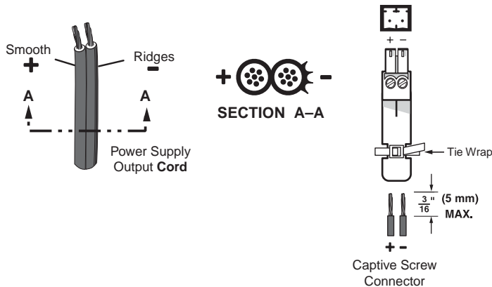
Figure 11. Power Connector Wiring
