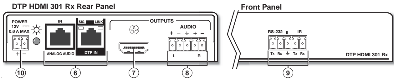
Figure 3. DTP HDMI 301 Rx Rear Panel Connectors
