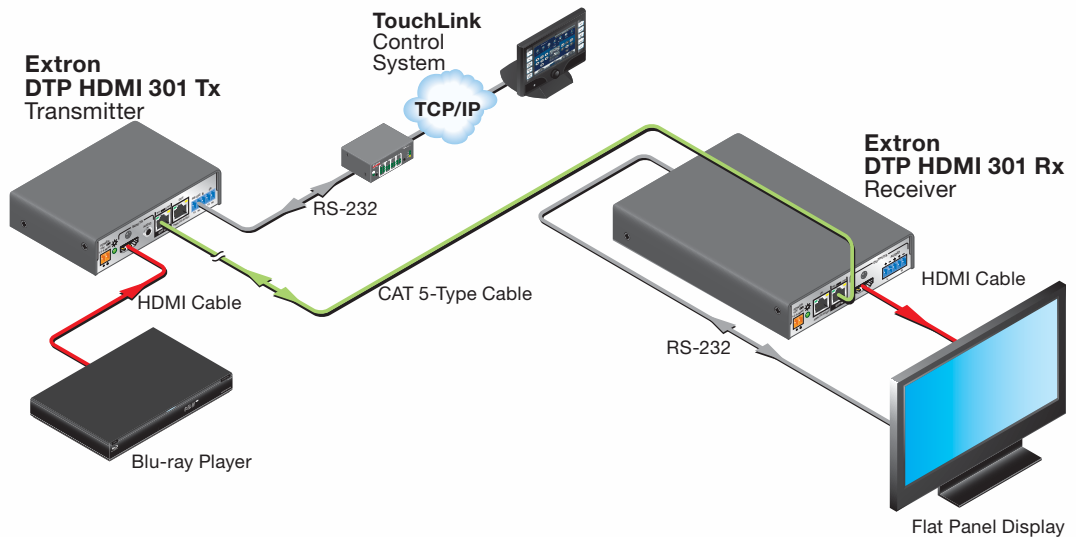
Figure 1. Typical Transmitter and Receiver Application
