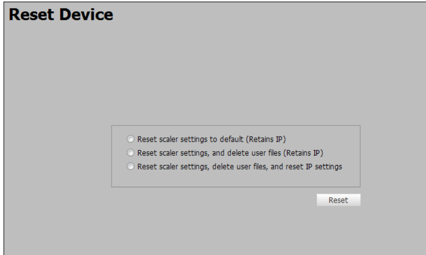
Figure 63. Password Page
