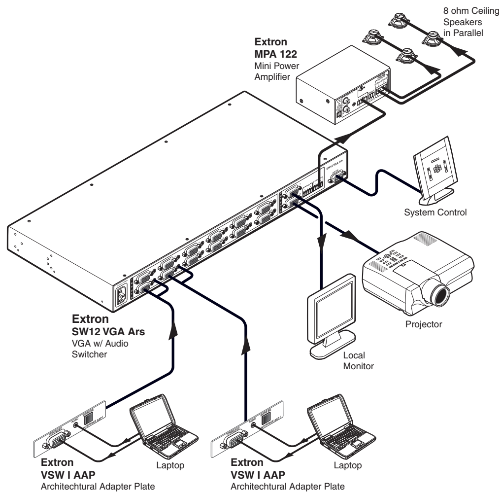
Figure 1-1 — A typical SW12 VGA Ars switcher application
