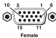
Figure 2-9 — Video output connectors
