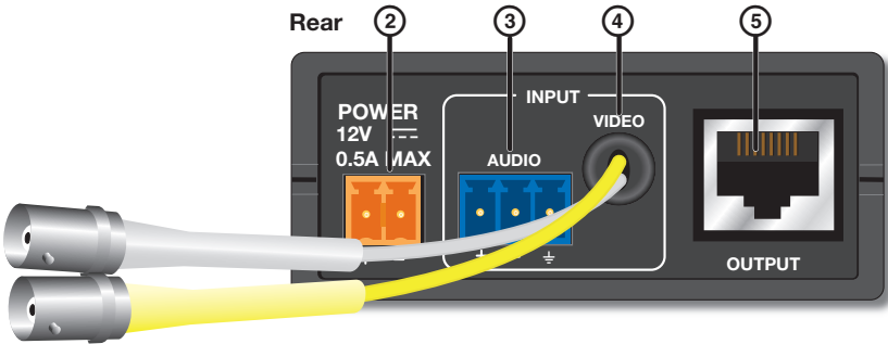
Figure 2. TLP VIM Front and Rear Panel
