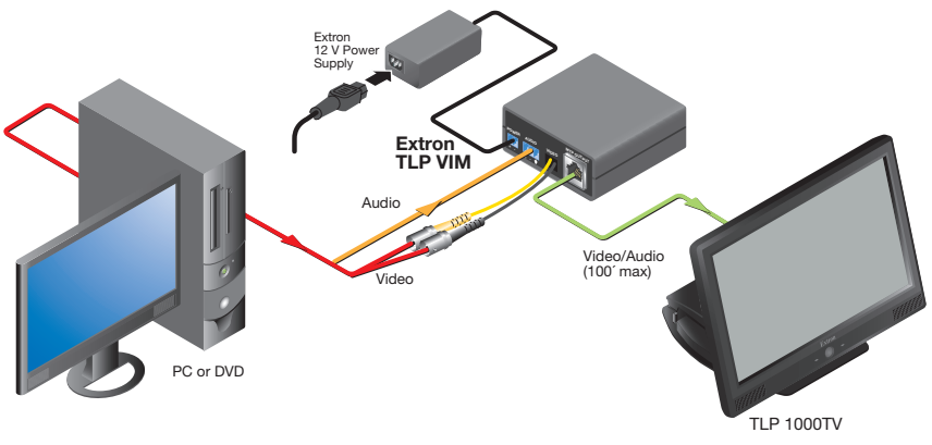
Figure 1. TLP VIM Application Diagrams
