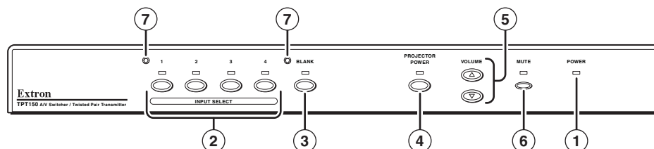
Figure 3-1 — TPT150 transmitter front panel
