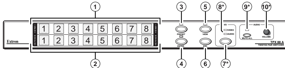
Figure 3-1 — TPX 88 A front panel
