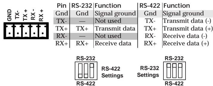
Figure 4-1 — Remote connector pin arrangement
