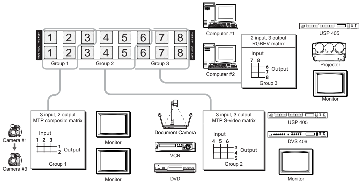
Figure 3-4 — I/O grouping of compatible twisted pair transmitter/receiver pairs
