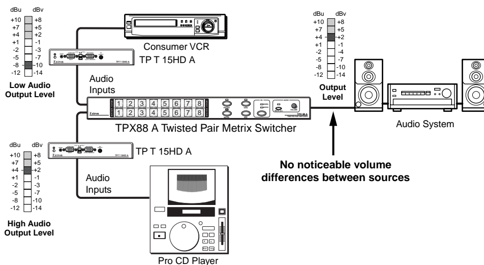
Figure 1-2 — Audio gain and attenuation
