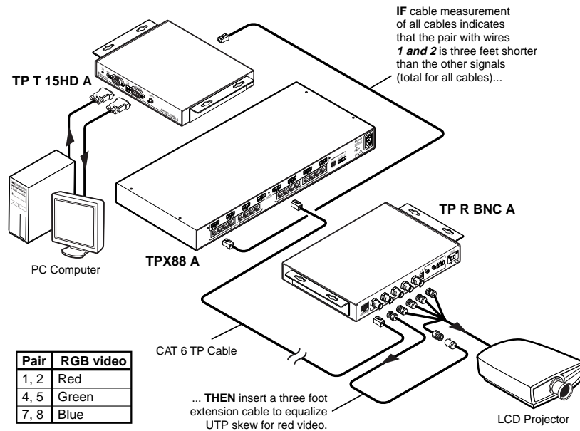
Figure 2-4 — Pair skew equalization
