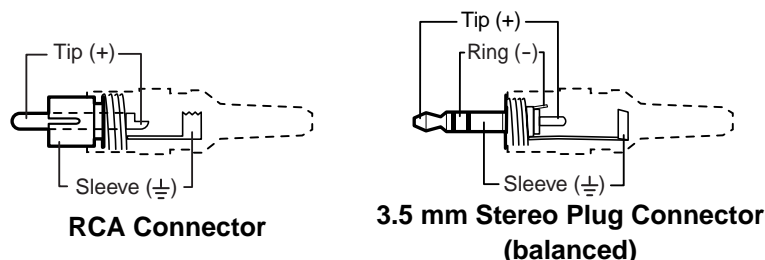
Figure 2-6 — Typical audio connectors
