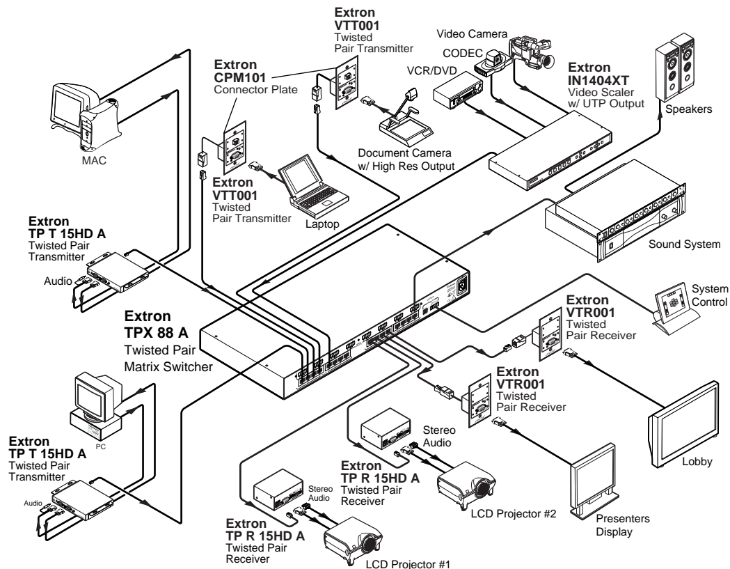
Figure 1-1 — Typical TPX 88 A matrix switcher application
