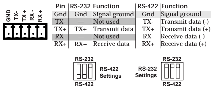
Figure 2-7 — Remote connector
