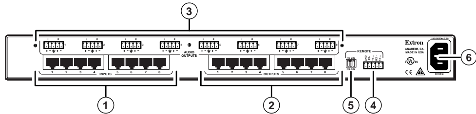
Figure 2-2 — TPX 88 A twisted pair matrix switcher with audio
