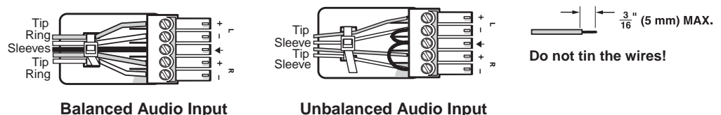
Figure 3. Audio Input Wiring
