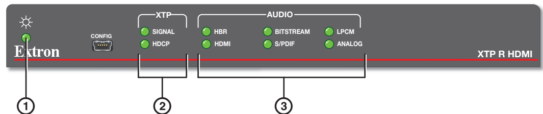
Figure 13. XTP R HDMI Front Panel Features
