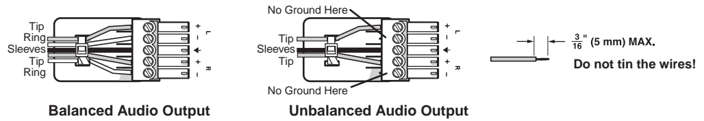
Figure 5. Audio Output Wiring
