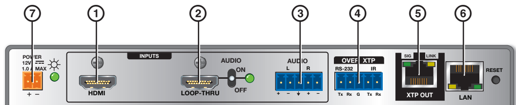
Figure 2. XTP T HDMI Rear Panel Connectors
