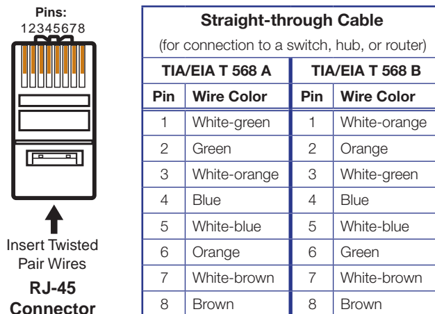
Figure 8. TP Cable Termination
