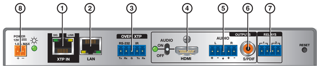
Figure 4. XTP R HDMI Connectors
