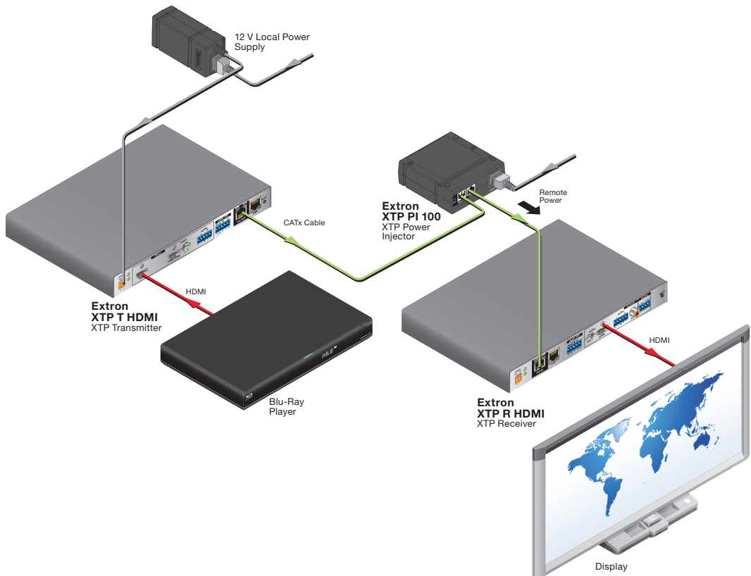
Figure 11. Typical Point-to-Point Application with Remote Power
