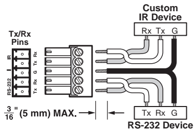
Figure 9. Wiring the RS-232 and IR Connector
