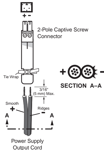
Figure 10. Power Wiring
