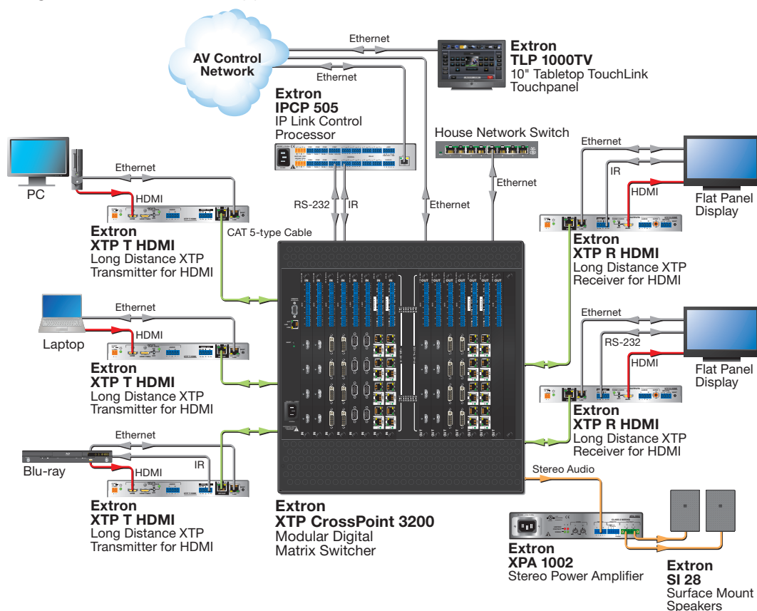
Figure 1. Typical XTP HDMI Transmitter and Receiver Matrix Application
