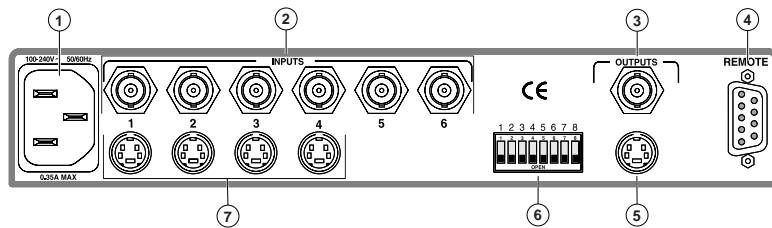
Figure 1 — YCS SW6 MX rear panel
